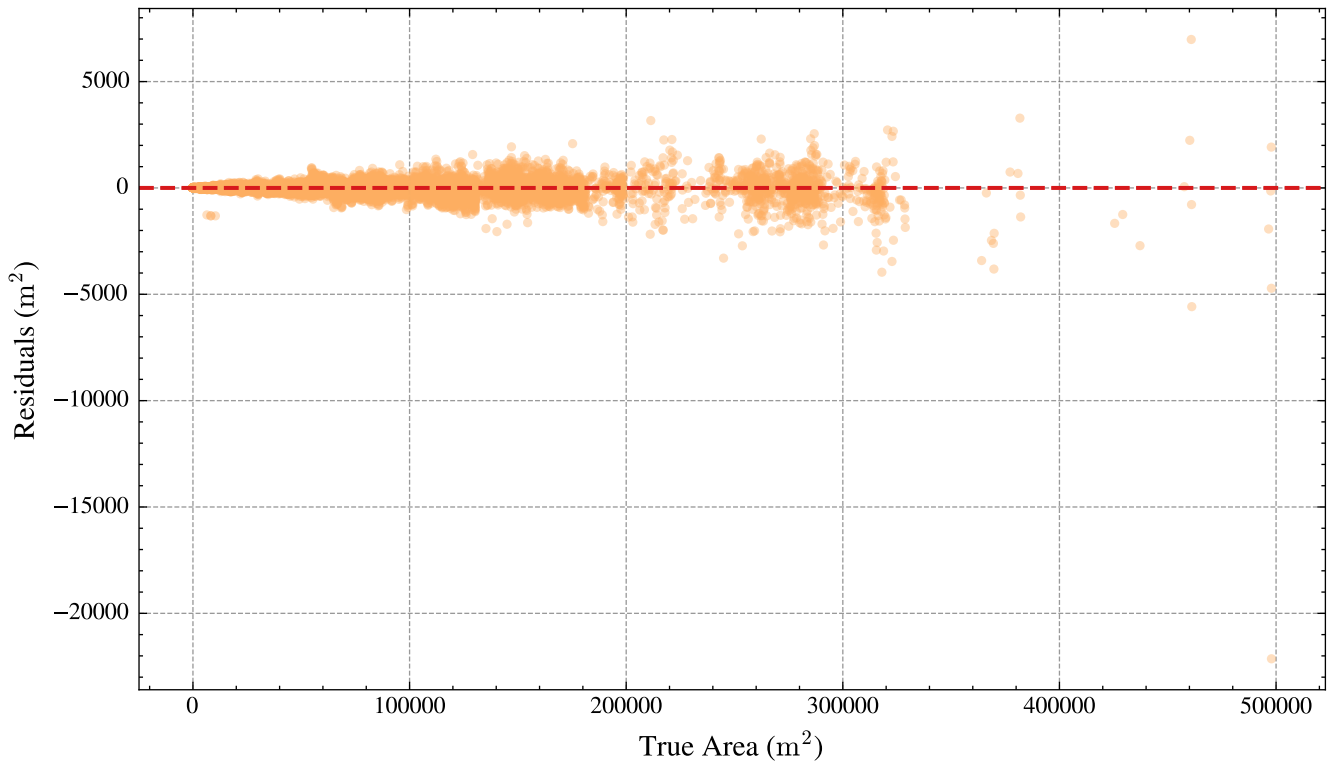
Optimized MLP — Residuals for Area
