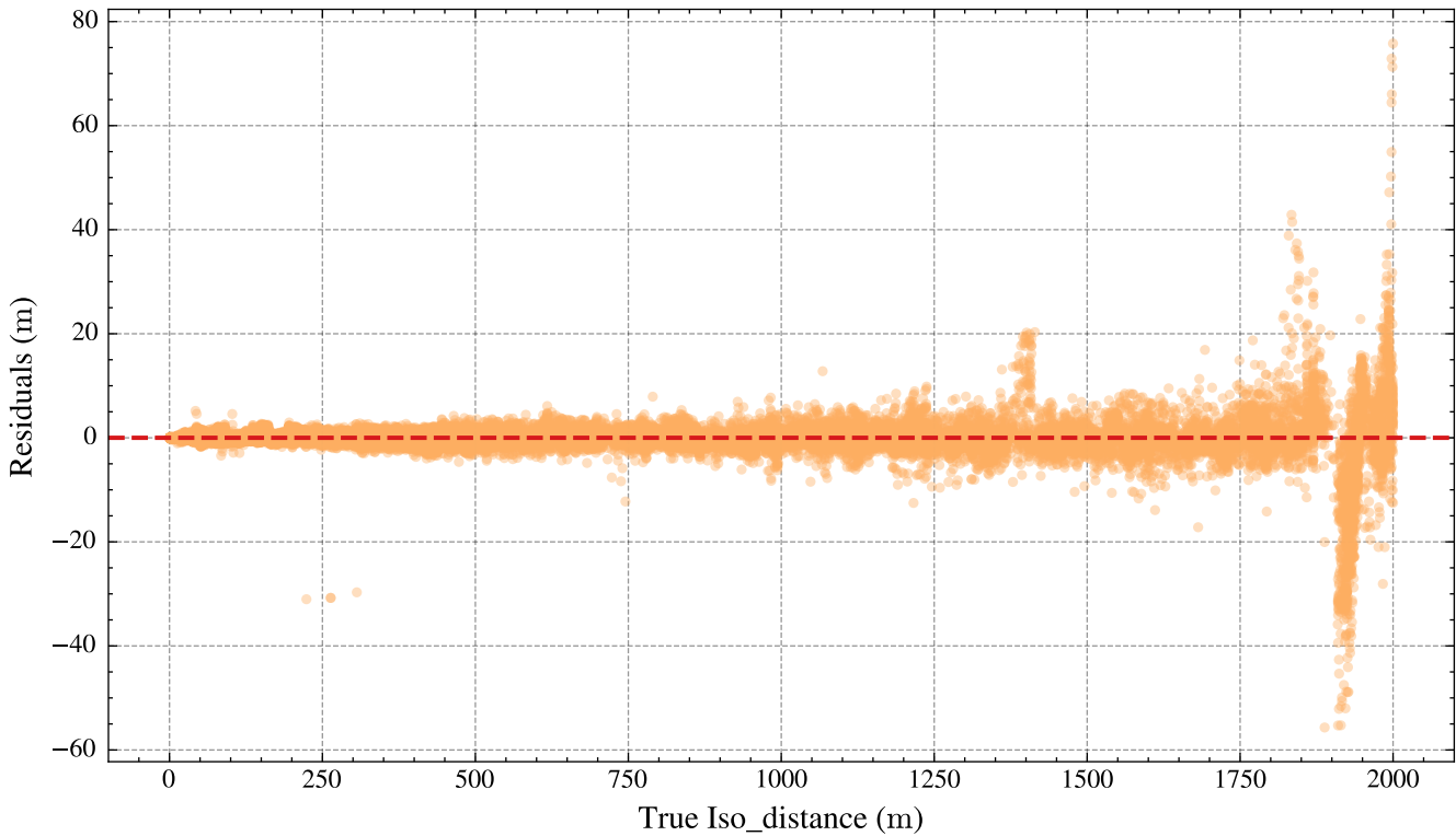
Optimized MLP — Residuals for Iso_distance
