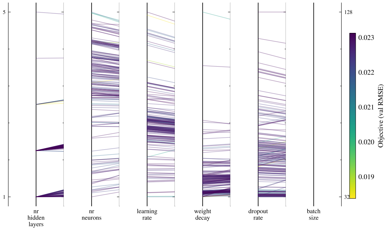
Parallel Coordinates — Top 200 Trials
