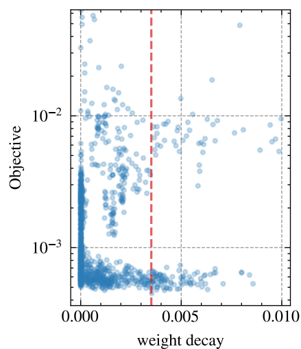
Objective vs. Hyperparameter (slice plots)
