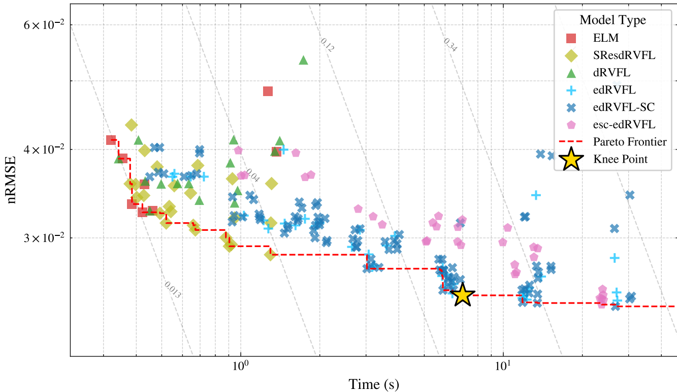
nRMSE vs. Training Time — Cone
