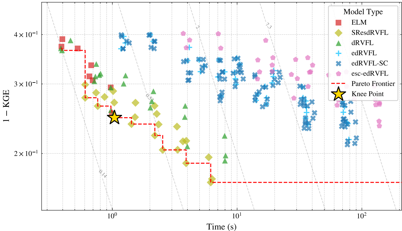
1 - KGE vs. Training Time — Isotherm
