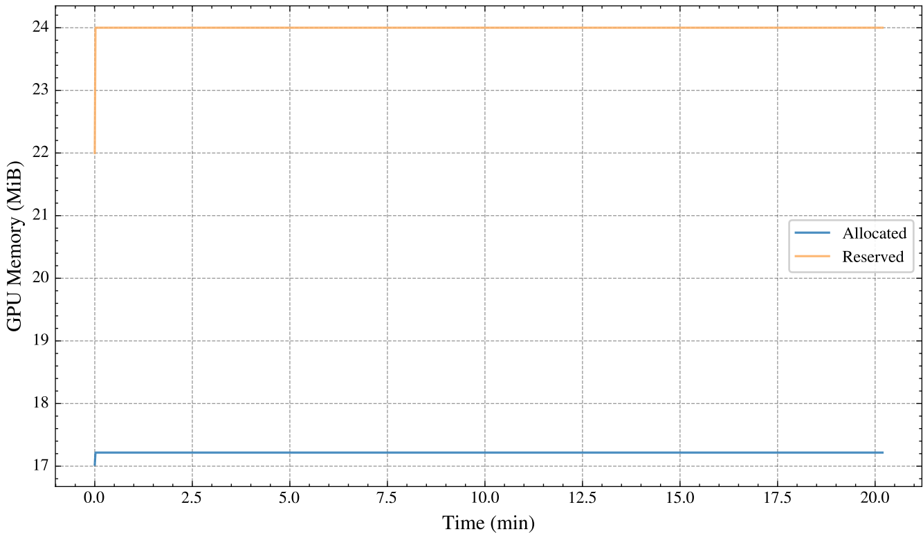
GPU Memory Usage — MLP Cone
