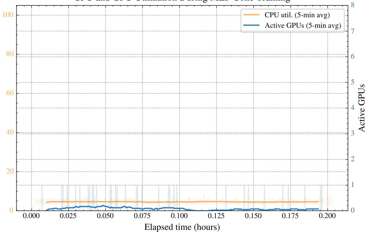
CPU and GPU Utilization During MLP Cone Training
