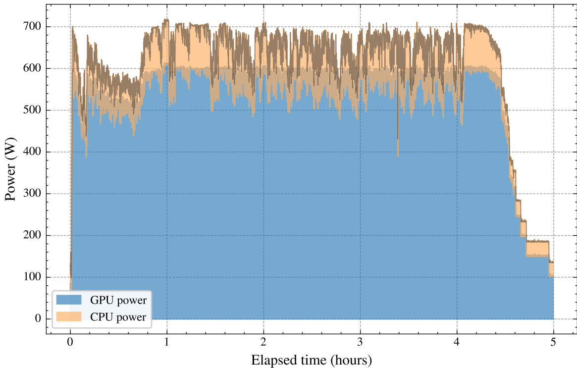
Node Power Consumption During Optuna Cone (run 1055)
