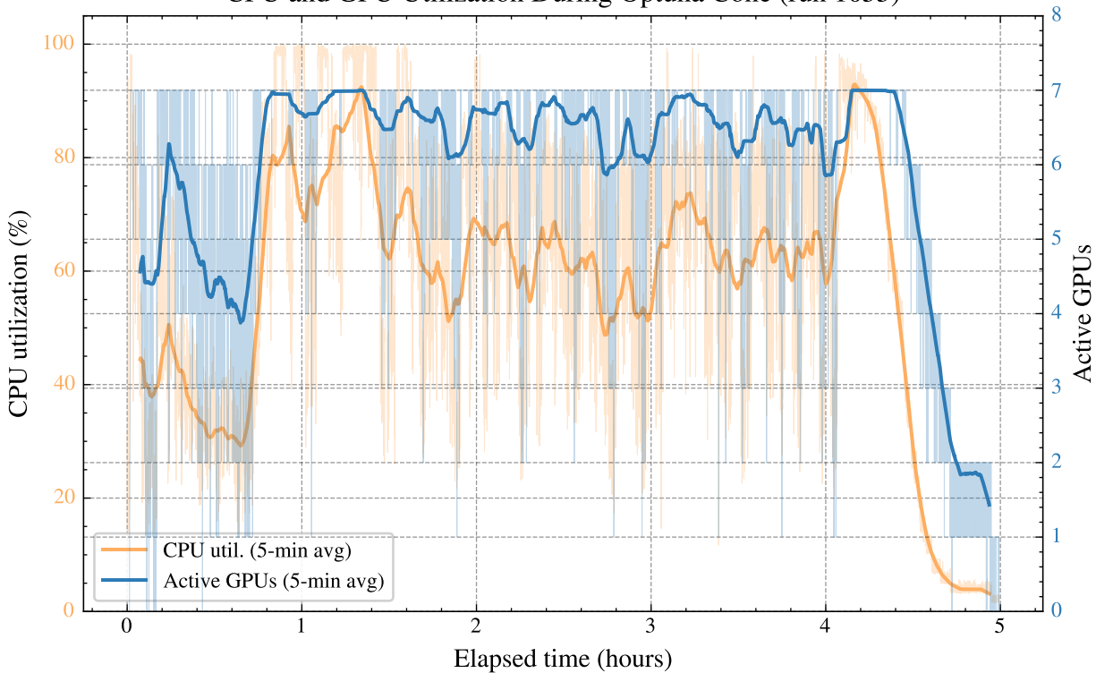
CPU and GPU Utilization During Optuna Cone (run 1055)
