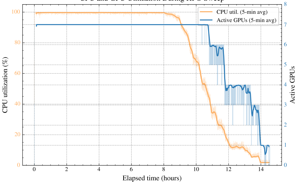
CPU and GPU Utilization During HPO Sweep
