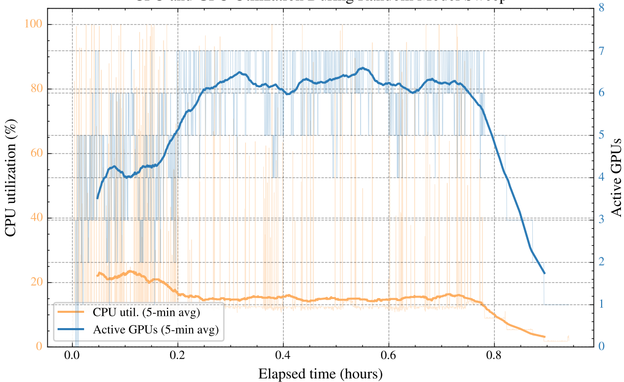
CPU and GPU Utilization During Random Model Sweep
