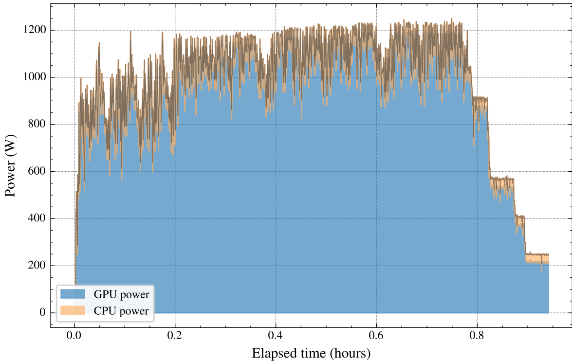
Node Power Consumption During Random Model Sweep
