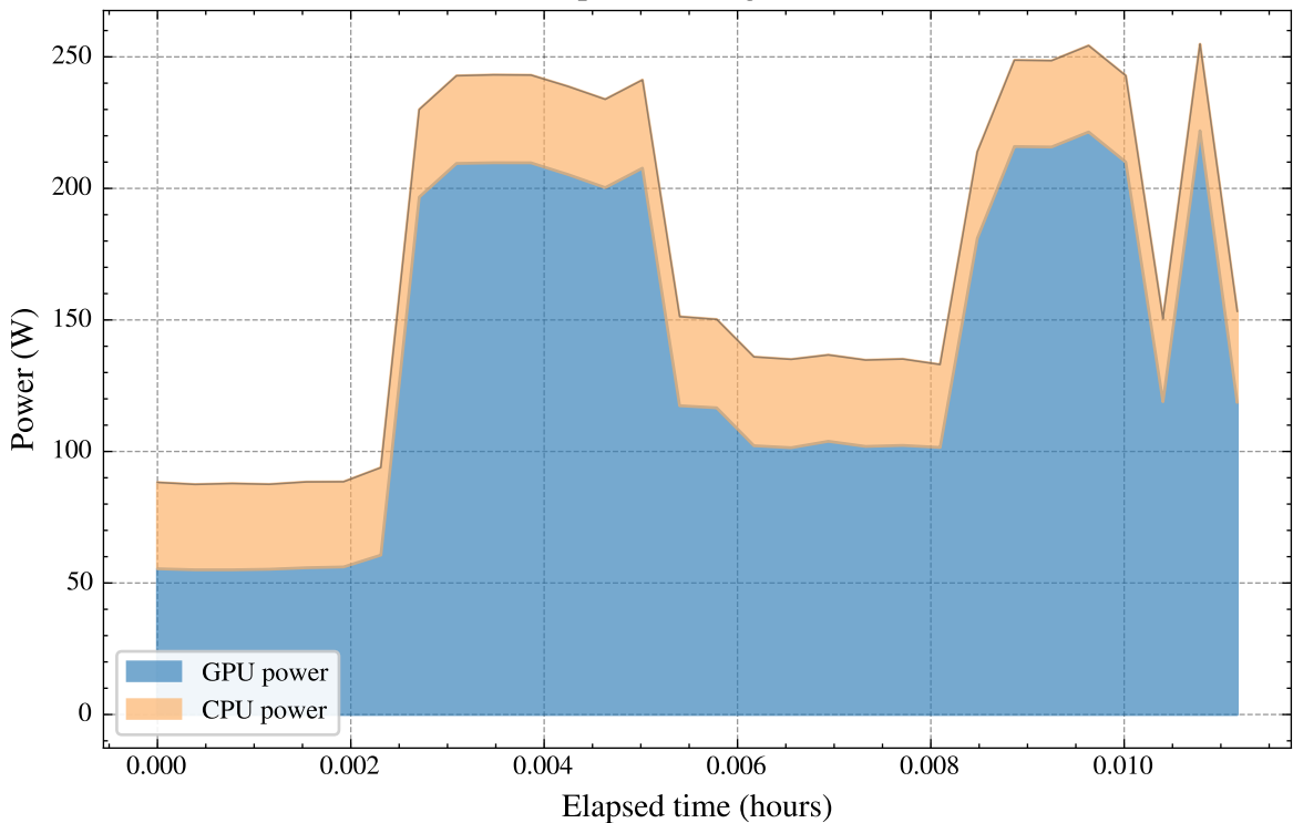
Node Power Consumption During Random Model Winners
