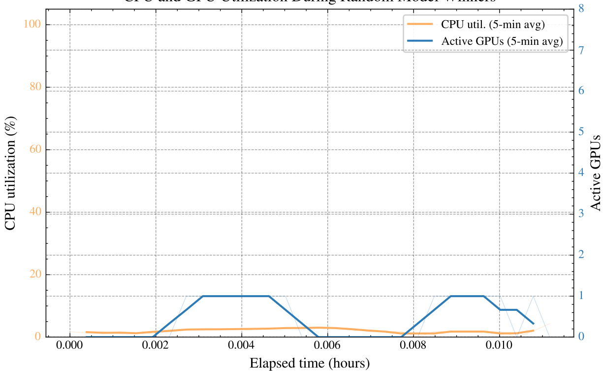
CPU and GPU Utilization During Random Model Winners
