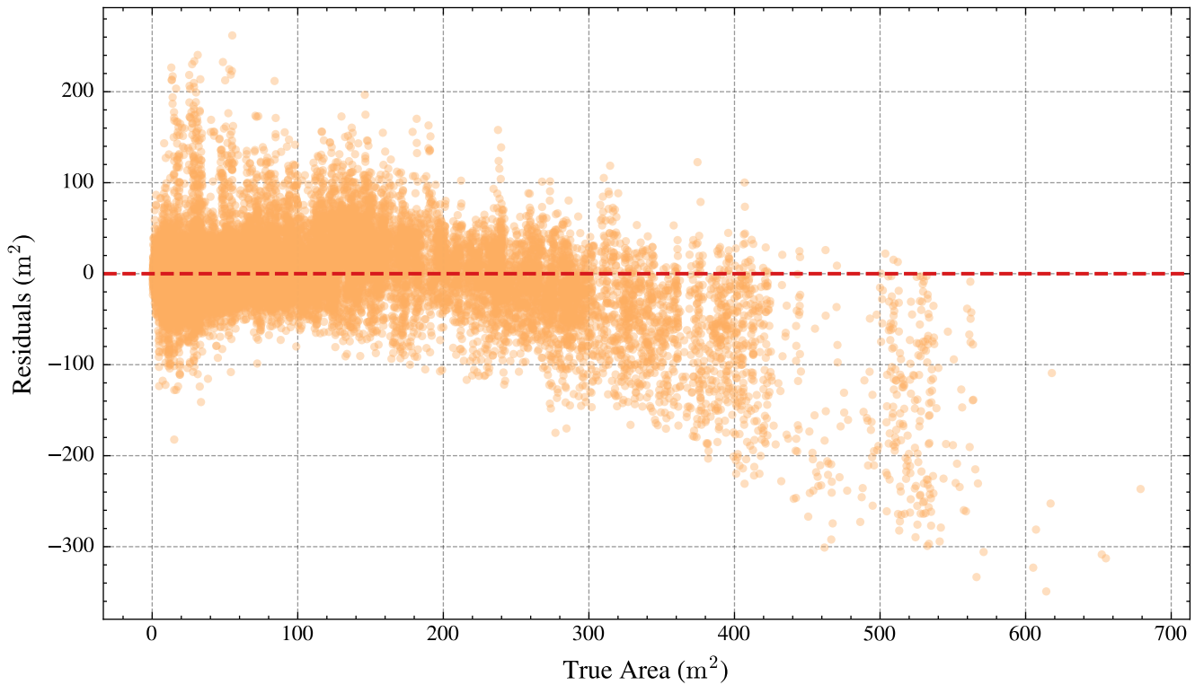
dRVFL (KGE winner) — Residuals for Area
