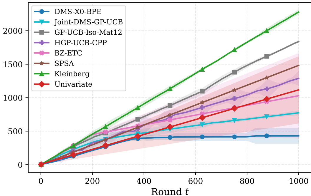
Complementary pricing — d = 6 , T = 1000 , 3 seeds
