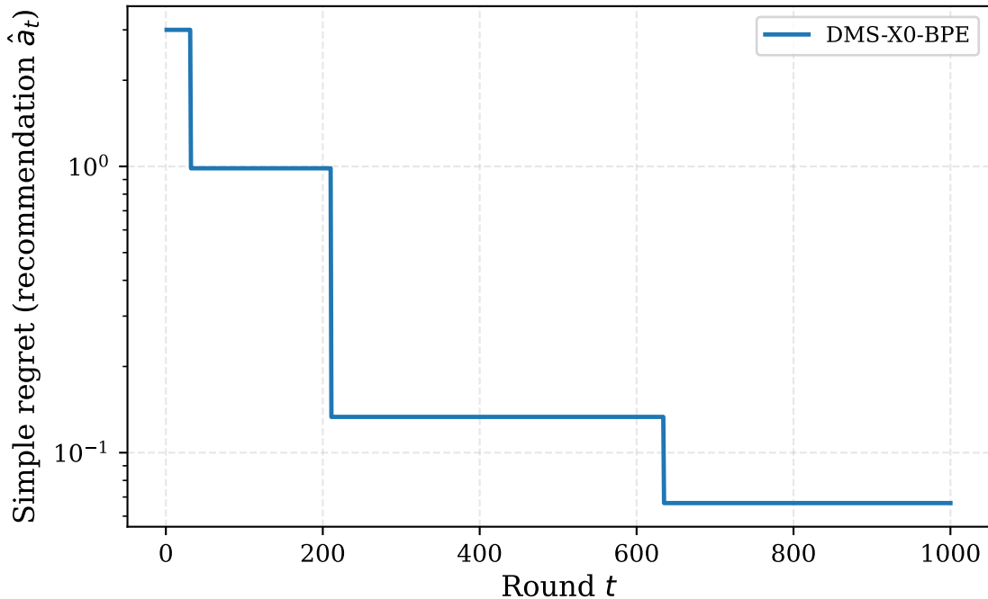
Complementary pricing — d = 6 , T = 1000 , 3 seeds
