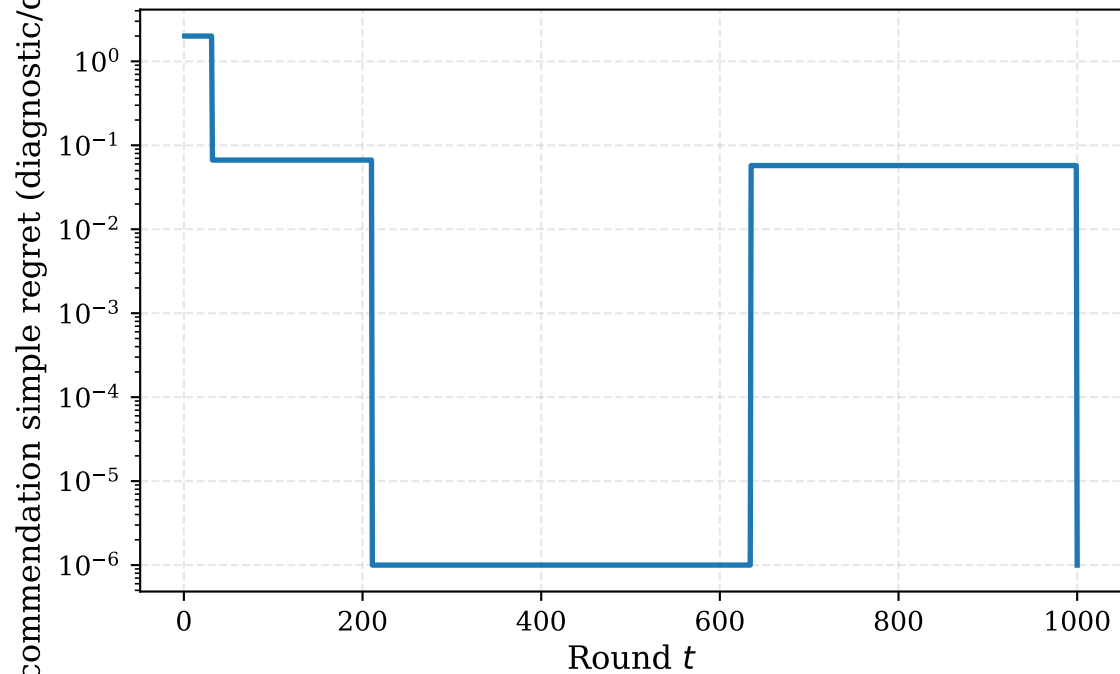
DMS-X0-BPE — T = 1000 , 3 seeds
