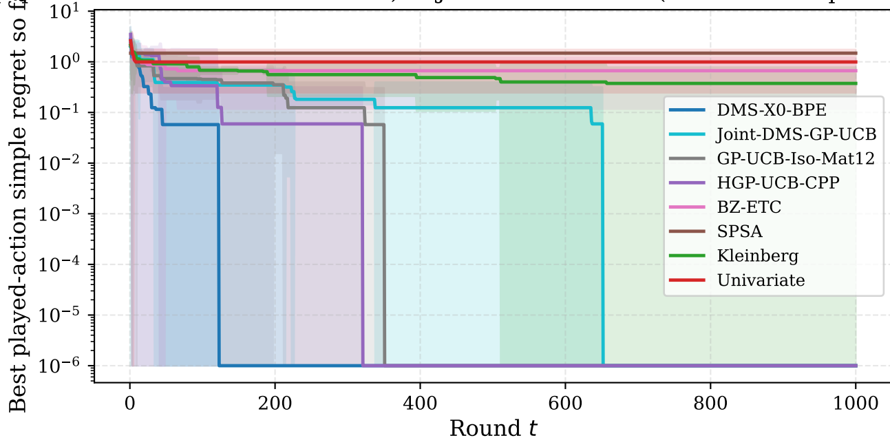
Complementary pricing — d = 6 , T = 1000 , 3 seeds
