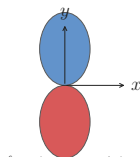
p_y orbital
