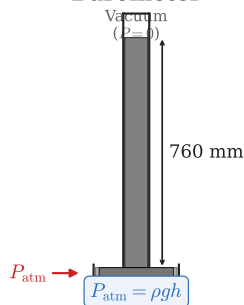
Barometer
