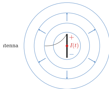
Oscillating Dipole Antenna EM waves radiate outward
