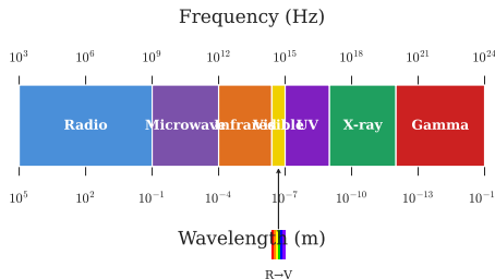
The Electromagnetic Spectrum
