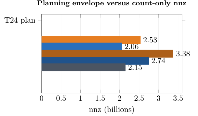
Fig. 2. Fail-closed resource evidence. T16 is a live-availability safety block, not a nominal 128-GB ceiling. T24 is a conservative policy-envelope block, not a demonstrated materialized overflow. T32 exceeds signed-int32 under both the envelope and count-only reconstruction. No row reached LP construction, solver allocation, or an OOM crash.
