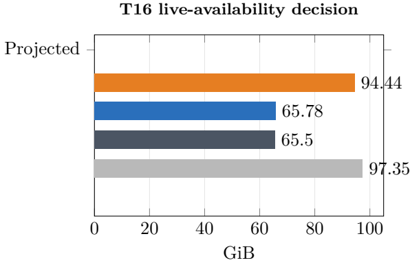
Fig. 2. Fail-closed resource evidence. T16 is a live-availability safety block, not a nominal 128-GB ceiling. T24 is a conservative policy-envelope block, not a demonstrated materialized overflow. T32 exceeds signed-int32 under both the envelope and count-only reconstruction. No row reached LP construction, solver allocation, or an OOM crash.
