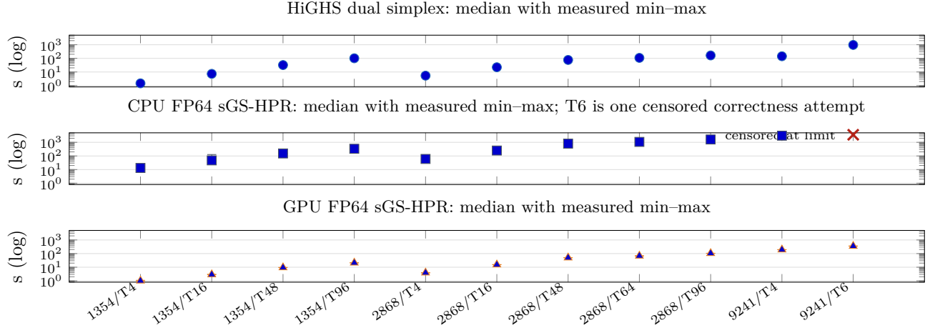
Fig. 1. Faceted local timing evidence. Each panel has a distinct solver definition; whiskers span measured minima and maxima. The plot supports within-track repeatability inspection only. Cross-solver ratios and speedups are not valid because the solver boundaries and algorithms differ.
