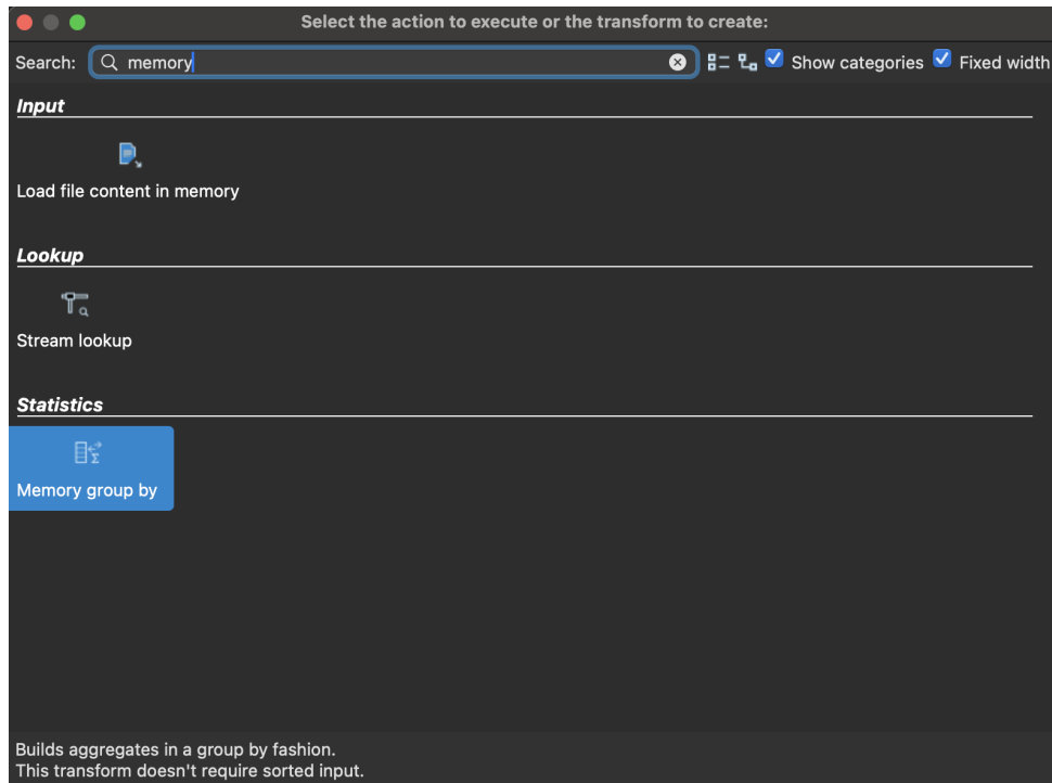
FIGURE 29 – Ajout de la transformation Memory group by .
