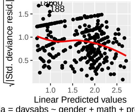
Scale-Location
