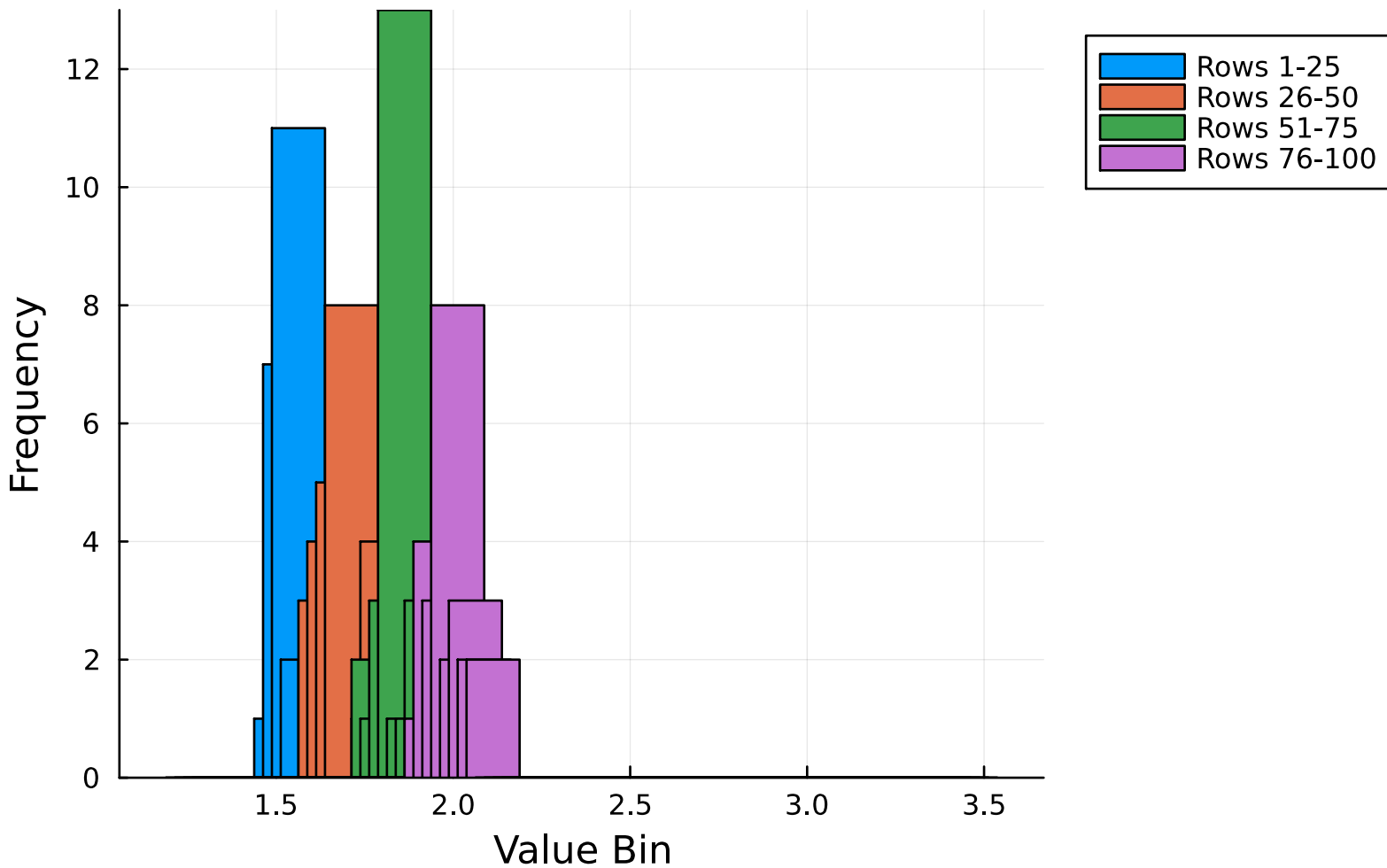
Comparison of Row Sets (Size 25)
