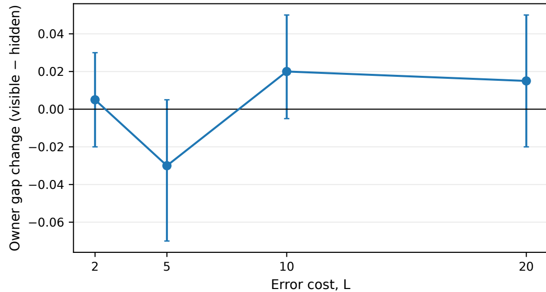
xai_grok420_nonreasoning
