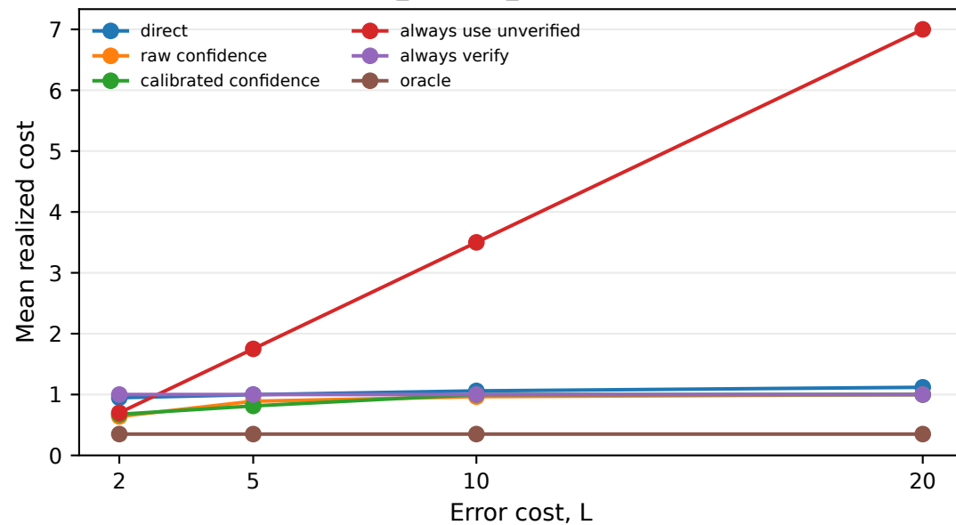
xai_grok420_nonreasoning
