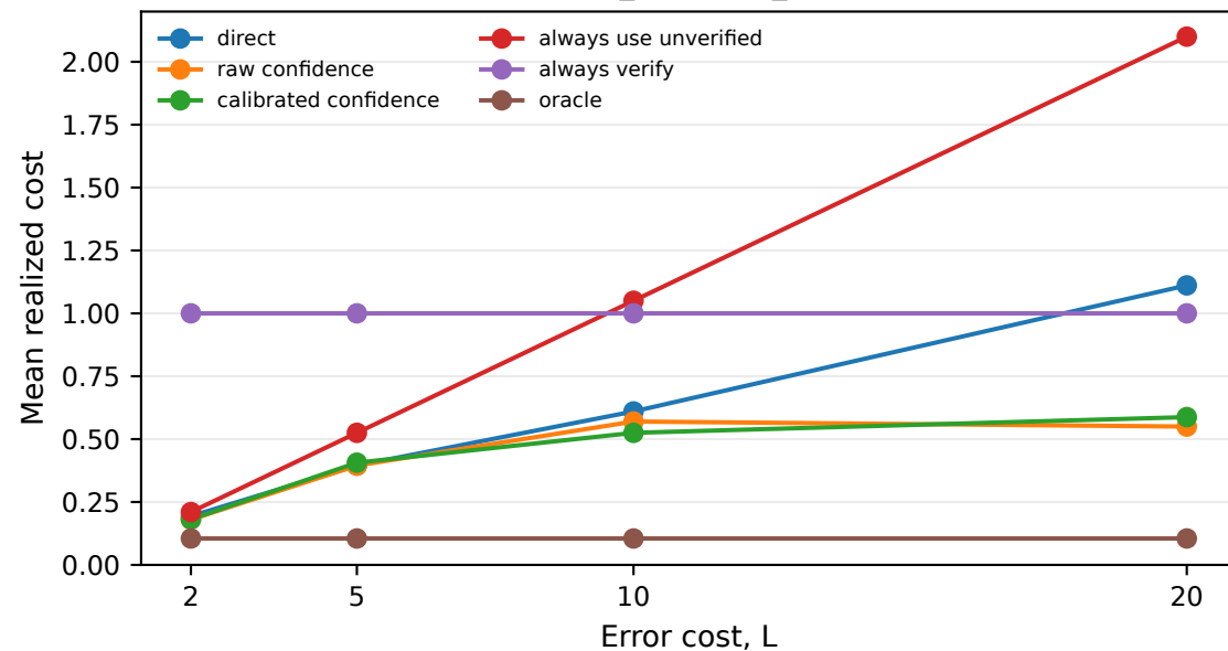
xai_grok420_nonreasoning
