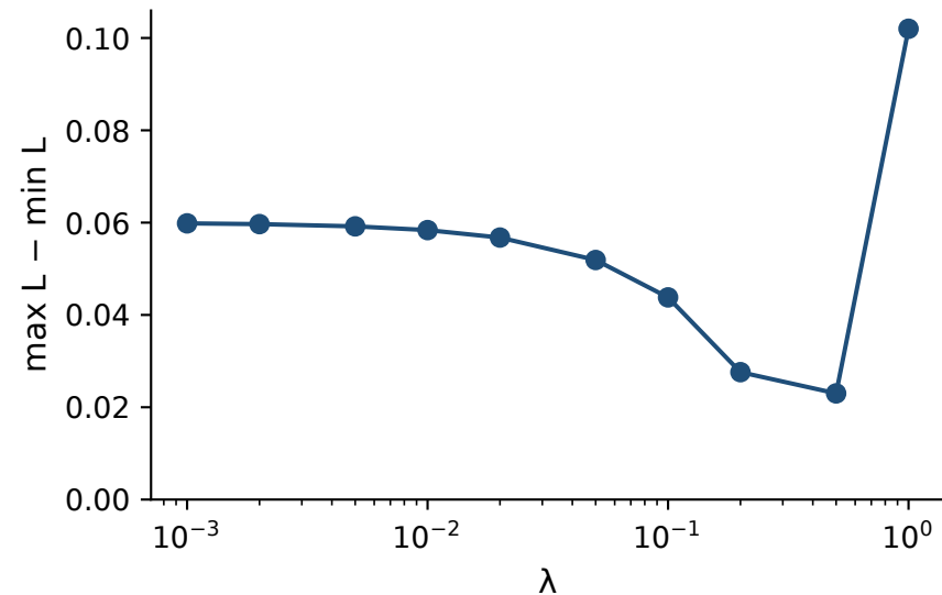
Claude MMLU-Pro
