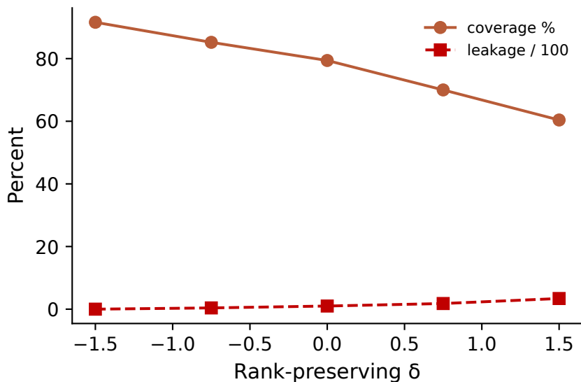
Claude MMLU-Pro
