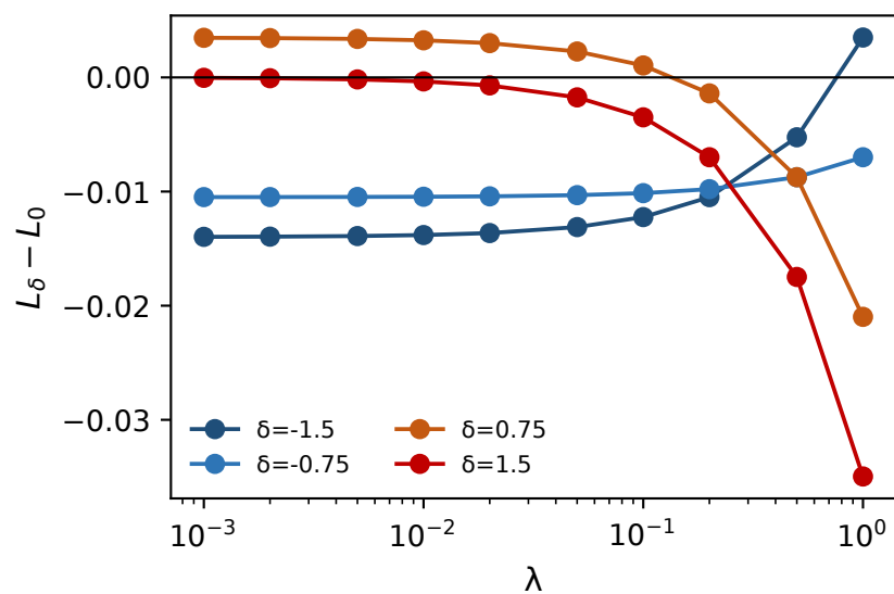
Claude LiveCodeBench
