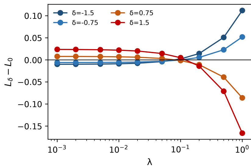
Claude MMLU-Pro
