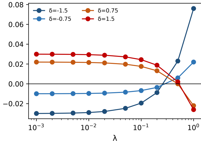
Claude MMLU-Pro
