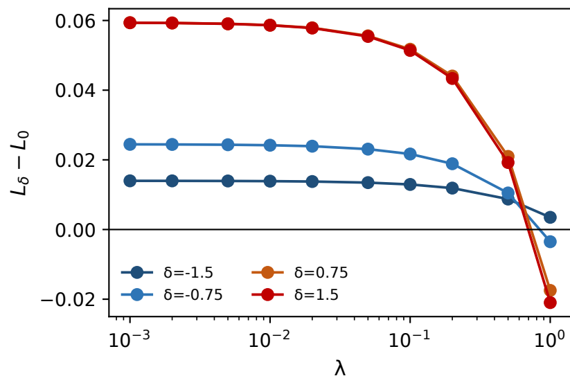
Claude LiveCodeBench
