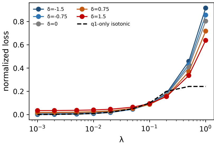
Claude MMLU-Pro
