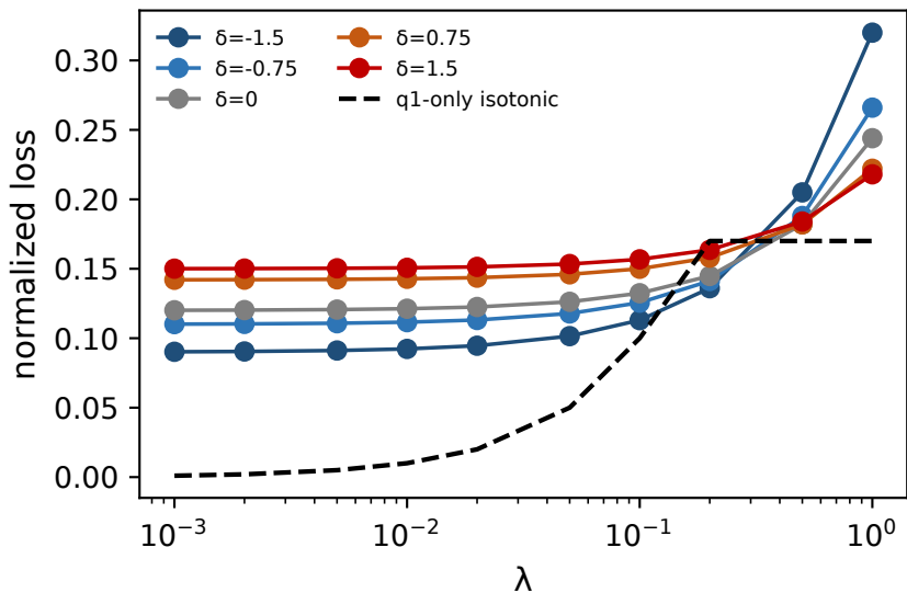
Claude MMLU-Pro
