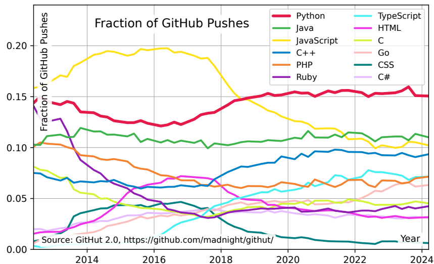
Figure 1.2: The twelve most popular programming languages chosen based on the GitHub pushes over the years. Source: [55].
