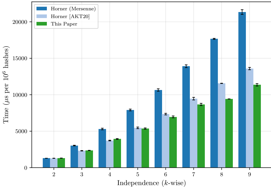
Mersenne Prime Field ( \mathbb{F}_{2^{89}-1} )
