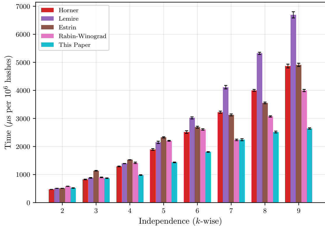
Carryless Multiplication ( \mathbb{F}_{2^{64}} )
