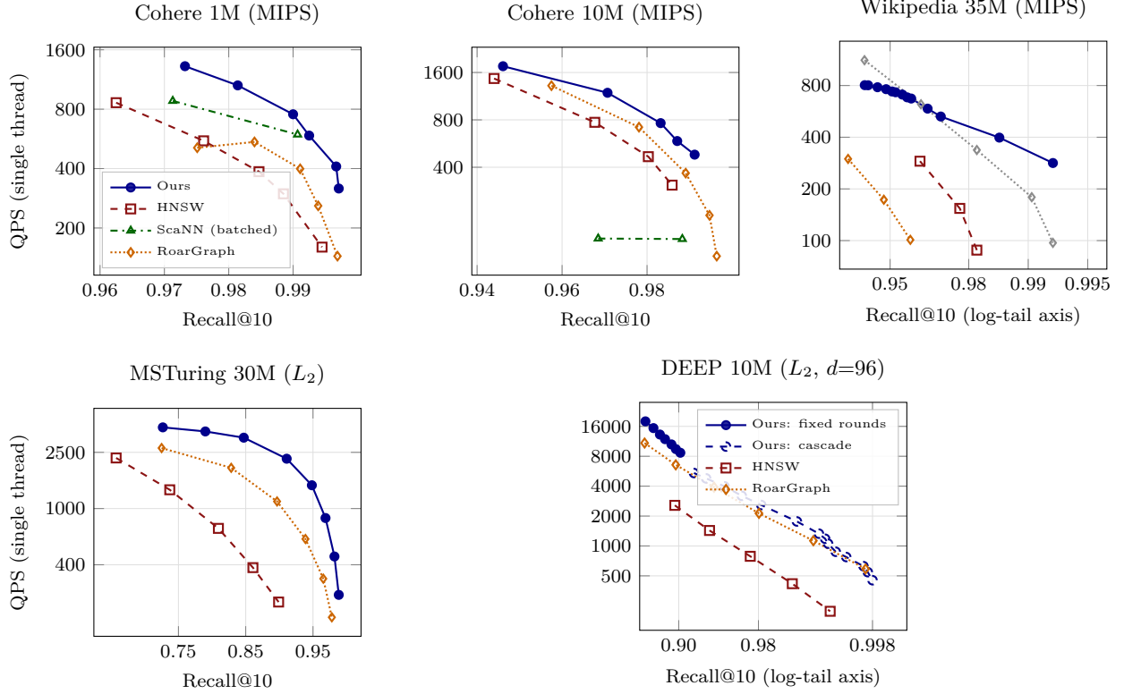
Figure 13: Recall-QPS frontiers (recall@10 versus single-thread queries per second, log scale). Every genbo curve uses the uniform full-query, highest-work-warmup, forward/reverse, best-of-five protocol with a 5% mirror-acceptance gate. Quoted ratios use same-core sequential pairs; in particular, the DEEP ratios below are strict ABBA/BAAB medians rather than ratios inferred from independently best plotted points. The Wikipedia and DEEP panels use a log-tail recall axis ( \log(1 - \text{recall}) , reversed) so the high-recall contest is resolved rather than compressed into the right edge; on Wikipedia the greyed curve is the build- ineligible 6.5h RoarGraph, the orange curve the gate-eligible budget RoarGraph. Top row (high-dimensional, d \geq 768 ): our regime. On Cohere 1M/10M ( d=768 ) our system leads every baseline using its best eligible configuration; RoarGraph, though it edges HNSW, is 1.6\text{--}2.4\times (1M) / 1.2\text{--}1.45\times (10M) behind us — its query-aware bipartite projection buys nothing when the query manifold is the base manifold. On Wikipedia 35M ( d=1024 ) our plotted curve is a 64-edge graph seeded from the k=16 pass — gate-eligible at 1.46 h total build — with the resident stack: it crosses even the 6.5h build- ineligible RoarGraph near recall 0.961 (0.9609@672 versus \sim 671 ), reaches 0.9677@587 versus \sim 565 , then leads by 1.10\times at 0.972, 1.61\times at 0.986, and 2.9\times at RoarGraph’s 0.9925 ceiling. It concedes only 0.93– \sim 0.961 (up to \sim 1.3\times at 0.933, narrowing to parity by 0.961) — an eligible-vs- ineligible comparison; a budget-matched RoarGraph ( L=50 , 250k train queries) still takes 3.1h and collapses to a 0.9605 ceiling at \sim 100 QPS, below our curve everywhere. We audited this conceded band with eight independent attack shapes — budgeted walks with portal entries, portal-seeded pools, two graph-to-cell voting schemes, a 288-configuration cascade grid, rank-256 navigation, a 2-bit scan rung (§12), and a 96-edge graph (whose edge-truncation ablation shows the gain is edge count , not quality) — and every one fails or washes by the same mechanism: at d=1024 a scattered candidate evaluation is first-touch bound, which is precisely the toll a pure graph search amortizes over a 6.5h build and a cascade cannot avoid at loose recall. We therefore report this band as a characterized boundary of the regime, not an open tuning gap. Bottom row (low-dimensional, d \leq 100 ). On MSTuring 30M ( d=100 ) we beat every baseline at every measured point ( 1.45\text{--}2.8\times RoarGraph, exceeding HNSW’s ceiling); RoarGraph’s curve required padding its input to d=104 — its released code silently corrupts dimensions not divisible by 8. On DEEP 10M ( d=96 ), graph-local physical ordering and corrected-fp16 reranking win the tail, while portal-SQ4 entry plus budgeted local refinement removes the loose routing+scan toll. Fixed rounds replace best-first above recall 0.80 and add 6.1–17.4% strict median QPS at matched recall; a direct pair at 0.9032 is 1.265\times RoarGraph ( 1.204\times best-to-best). Ours beats RoarGraph across the loose curve and by strict same-window medians of 1.19\text{--}1.38\times from 0.943 through 0.994, reaching a reproduced 0.9980 beyond its ceiling. The two genbo mechanisms are separate plotted series: no line interpolates across the unmeasured 0.9032–0.9265 gap. The 0.9265 join shoulder and the 0.9978 point remain inside RoarGraph’s demonstrated \sim 1.2\times window-phase swing and are marked parity pending multi-window confirmation; the 0.9032 join point itself is confirmed across three window-separated quiet ABBA rounds (medians 1.09\times , nearly behind under any arithmetic convention).
