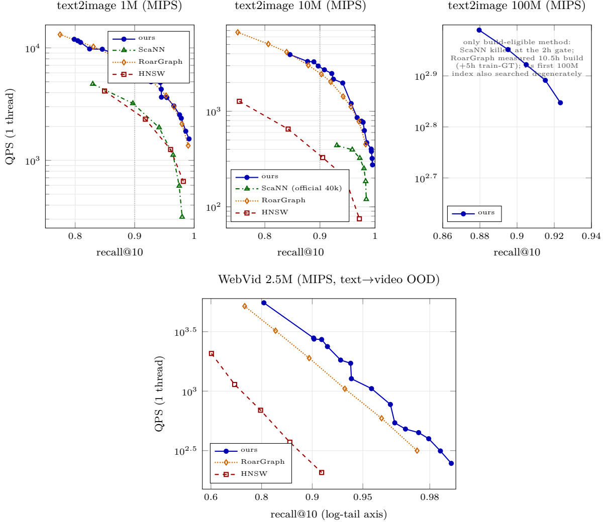
Figure 14: Out-of-distribution frontiers (text2image, d=200 , inner product): QPS vs. recall@10, single thread, same box, at 1M, 10M, and 100M. Ours, ScaNN, and RoarGraph are per-query sweeps (mode-matched; ScaNN’s batched API amortizes a further \sim 3\text{--}4\times and is then competitive with our per-query cascade above recall \approx 0.96 at 10M); HNSW runs in its batched API (favorable to HNSW). Ours sweeps probe depth at hops 2–4 with the self-built k=16 graph ( k=32 at the tail). Ours uses the hybrid graph — 16 base- k NN edges + 16 co-retrieval edges (bipartite projection of the track’s training queries, the same resource RoarGraph consumes; §17) — as a drop-in adjacency file. At the leaderboard gate (recall 0.90, dotted), ours leads at 10M ( 1.25\times RoarGraph per-query, 6.5\times ScaNN, 8.7\times HNSW), leads the entire measured 10M range through recall 0.9954 (best-first beam over the hybrid edges; 0.9931 at 402 QPS vs RoarGraph’s 0.9905 at 322), and is the only eligible method at 100M; at 1M, applying the coarse-cell corollary ( K_f=16384 \rightarrow 2048\text{--}4096 ; graph coverage replaces fine partitioning, §8) closes the band: ours ties or leads RoarGraph from recall \approx 0.80 upward (gate: 6.6k vs 6.4k QPS) and takes the 1M tail (0.9914 at 1551 vs 0.9900 at 1353); RoarGraph stays marginally ahead only below recall \approx 0.78 . A code-side IVPQ-FastScan+refine baseline caps at recall 0.73 (10M) and does not appear. The bottom panel adds WebVid ( d=512 ), RoarGraph’s hardest published benchmark and an extreme -OOD regime: calibrated routed coverage reaches only 0.36 at p=32 (vs 0.83 on text2image), so nearly all coverage must come from materialized adjacency. An oracle decomposition (perfect seeds \Rightarrow recall 1.0 at minimal configs) shows the gap is purely seed coverage, and two levers close it: dense query-seeds (each test query’s nearest training queries vote their materialized ground-truth answers as entry seeds, both using the same training resource RoarGraph consumes; coverage 0.42 \rightarrow 0.76 ) and a resident 4-bit scoring rung (per-dim scalar-quantized nibbles, d/2 bytes/row, rank-exact via query-side step folding, int8 re-rank of the top band), plus a wide hybrid graph for the loose corner (16 base- k NN + 48 co-retrieval edges, built in 11s). With these, ours beats RoarGraph at every measured point of its curve: 1.3\times at recall 0.81, 1.5\times at 0.90, 1.7\times at 0.91, 1.6\times at 0.92–0.93, 1.2\times at 0.963, ahead through 0.985 — past its ceiling on its own benchmark. All genbo panels use the uniform full-query protocol: highest-work warmup, exact forward/reverse plan, five inner repetitions, and acceptance only when every mirrored QPS pair is within 5%. The two WebVid loosest points reproduce within 2%, while all points \geq 0.92 are stable across every measured window. RoarGraph’s curve is its own quiet-window best.
