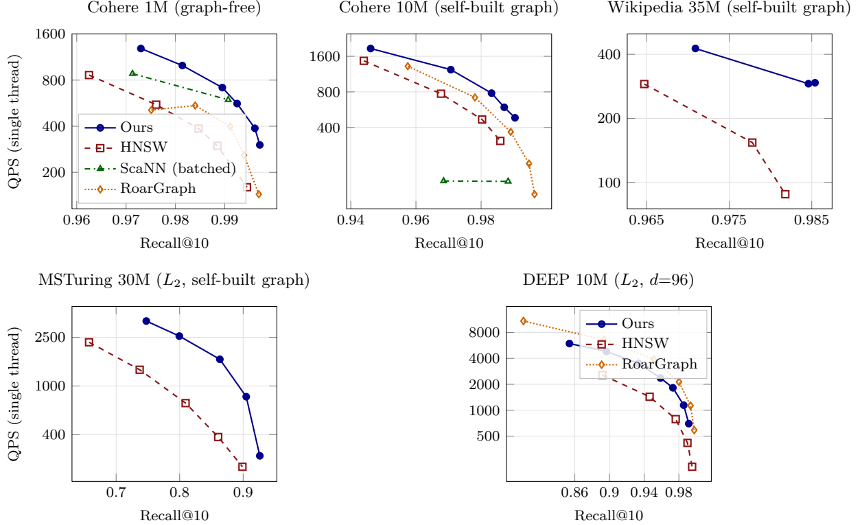
Figure 13: Recall-QPS frontiers (recall@10 versus single-thread queries per second, log scale), same-window sequential pairs. Top row (high-dimensional, d \geq 768 ): our regime. On Cohere 1M/10M ( d=768 ) and Wikipedia 35M ( d=1024 ) our system leads every baseline — graph-free at 1M and with self-built graphs at 10M/35M; HNSW plateaus at recall 0.9945/0.9859/0.9818 below what we reach, ScaNN (batched, favorable to it) trails, and RoarGraph, though it edges HNSW, is 1.6\text{--}2.4\times (1M) / 1.2\text{--}1.45\times (10M) behind us — its query-aware bipartite projection buys nothing when the query manifold is the base manifold. Bottom row (low-dimensional, d \leq 100 ): the boundary. On MSTuring 30M ( d=100 ) and DEEP 10M ( d=96 ) our system still beats HNSW ( 2.5\text{--}4\times / \sim 2\times , exceeding HNSW’s ceiling on MSTuring) and ScaNN, but a strong pure graph index (RoarGraph) leads DEEP by 1.3\text{--}1.7\times : at low dimension the value of PQ compression and coverage augmentation shrinks while cheap graph traversal dominates. Our advantage is thus the high-dimensional embedding regime; the crossover near d \sim 100 is where graph indices reclaim the frontier. (RoarGraph’s harness mis-counts recall on MSTuring’s large-magnitude L_2 distances, so only its DEEP curve is shown.)
