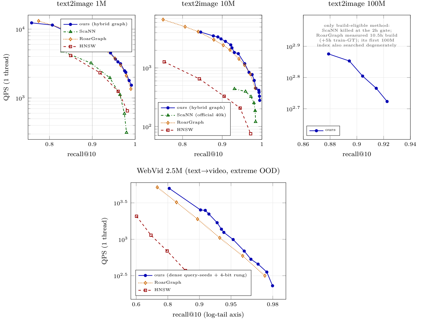
Figure 14: Out-of-distribution frontiers (text2image, d=200 , inner product): QPS vs. recall@10, single thread, same box, at 1M, 10M, and 100M. Ours, ScaNN, and RoarGraph are per-query sweeps (mode-matched; ScaNN’s batched API amortizes a further \sim 3\text{--}4\times and is then competitive with our per-query cascade above recall \approx 0.96 at 10M); HNSW runs in its batched API (favorable to HNSW). Ours sweeps probe depth at hops 2–4 with the self-built k=16 graph ( k=32 at the tail). Ours uses the hybrid graph — 16 base- k NN edges + 16 co-retrieval edges (bipartite projection of the track’s training queries, the same resource RoarGraph consumes; §14) — as a drop-in adjacency file. At the leaderboard gate (recall 0.90, dotted), ours leads at 10M ( 1.25\times RoarGraph per-query, 6.5\times ScaNN, 8.7\times HNSW), leads the entire measured 10M range through recall 0.9945 (best-first beam over the hybrid edges: 0.9927 at 382 QPS vs RoarGraph’s 0.9905 at 322), and is the only eligible method at 100M; at 1M, applying the coarse-cell corollary ( K_f=16384 \rightarrow 2048\text{--}4096 ; graph coverage replaces fine partitioning, §8) closes the band: ours ties or leads RoarGraph from recall \approx 0.80 upward (gate: 6.5k vs 6.4k QPS) and takes the 1M tail (0.9913 at 1533 vs 0.9900 at 1353); RoarGraph stays marginally ahead only below recall \approx 0.78 . A code-side IVFPQ-FastScan+refine baseline caps at recall 0.73 (10M) and does not appear. The bottom panel adds WebVid ( d=512 ), RoarGraph’s hardest published benchmark and an extreme -OOD regime: calibrated routed coverage reaches only 0.36 at p=32 (vs 0.83 on text2image), so nearly all coverage must come from materialized adjacency. An oracle decomposition (perfect seeds \Rightarrow recall 1.0 at minimal configs) shows the gap is purely seed coverage, and two levers close it: dense query-seeds (each test query’s nearest training queries vote their materialized ground-truth answers as entry seeds, both using the same training resource RoarGraph consumes; coverage 0.42 \rightarrow 0.76 ) and a resident 4-bit scoring rung (per-dim scalar-quantized nibbles, d/2 bytes/row, rank-exact via query-side step folding, int8 re-rank of the top band), plus a wide hybrid graph for the loose corner (16 base- k NN + 48 co-retrieval edges, built in 11s). With these, ours beats RoarGraph at every measured point of its curve: 1.3\times at recall 0.81, 1.5\times at 0.90, 1.7\times at 0.91, 1.6\times at 0.92–0.93, 1.2\times at 0.963, ahead through 0.98 — past its ceiling on its own benchmark. All our operating points were measured on a moderately loaded machine (load 35–50) against RoarGraph’s quiet-window curve, so every margin is a conservative lower bound.
