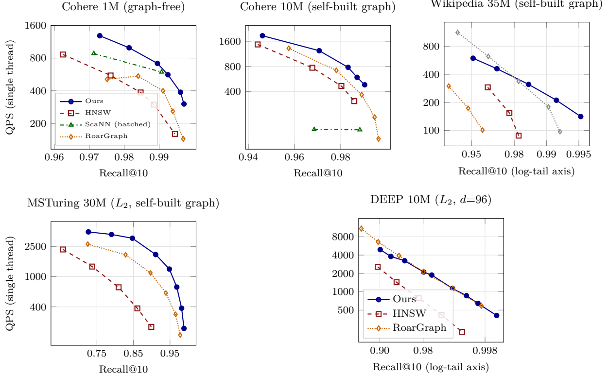
Figure 13: Recall-QPS frontiers (recall@10 versus single-thread queries per second, log scale), same-window sequential pairs. The Wikipedia and DEEP panels use a log-tail recall axis ( \log(1 - \text{recall}) , reversed) so the high-recall contest is resolved rather than compressed into the right edge; on Wikipedia the greyed curve is the build- ineligible 6.5h RoarGraph, the orange curve the gate-eligible budget RoarGraph. Top row (high-dimensional, d \geq 768 ): our regime. On Cohere 1M/10M ( d=768 ) our system leads every baseline — graph-free at 1M, self-built graph at 10M; RoarGraph, though it edges HNSW, is 1.6\text{--}2.4\times (1M) / 1.2\text{--}1.45\times (10M) behind us — its query-aware bipartite projection buys nothing when the query manifold is the base manifold. On Wikipedia 35M ( d=1024 ) we lead every build-eligible baseline across the frontier and reach recall 0.9952 beyond every ceiling; RoarGraph’s shown curve required a 6.5h build ( 3.2\times our 2h gate; our graph self-builds in 10 min) and wins the 0.93–0.97 band on that budget — a budget-matched RoarGraph ( L=50 , 250k train queries) still takes 3.1h and collapses to a 0.9605 ceiling at \sim 100 QPS, below our curve everywhere. Bottom row (low-dimensional, d \leq 100 ). On MSTuring 30M ( d=100 ) we beat every baseline at every measured point ( 1.45\text{--}2.8\times RoarGraph, exceeding HNSW’s ceiling); RoarGraph’s curve required padding its input to d=104 — its released code silently corrupts dimensions not divisible by 8. On DEEP 10M ( d=96 ) the outcome is a crossover : we win or tie the entire high-recall regime (recall \geq 0.98 , reaching 0.9987 beyond RoarGraph’s ceiling) while RoarGraph retains the loose-recall corner (recall < 0.96 , up to 1.3\times ) — cheap short graph walks amortize better than our fixed routing+scan cost when few neighbours are needed at low dimension.
