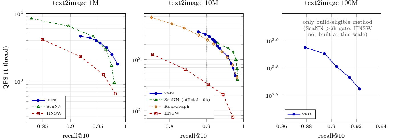
Figure 14: Out-of-distribution frontiers (text2image, d=200 , inner product): QPS vs. recall@10, single thread, same box, at 1M, 10M, and 100M. Ours is a per-query probe-depth sweep (hops 2–3; below the \approx 0.91 hop crossover this slightly understates our frontier, §7); ScaNN and HNSW run in their batched APIs (batching amortizes their per-query cost \sim 3\text{--}4\times — measured per-query, ScaNN’s 10M curve drops from 1396 to 323 QPS at recall 0.972 — so the baseline curves are favorable to the baselines); RoarGraph uses its own harness at one thread. At the leaderboard gate (recall 0.90, dotted) ours leads every system at every scale. Above recall \approx 0.96 at 10M, batch-mode ScaNN (deep reorder) and RoarGraph become competitive with our per-query cascade — genbo’s OOD advantage is the gate-to-0.95 band — while HNSW trails everywhere below its 0.97 tail. At 100M no baseline clears the 2h build gate, so ours is the only curve. A code-side IVFPQ-FastScan+refine baseline caps at recall 0.73 (10M) and does not appear.
