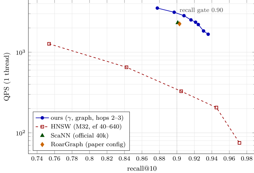
Figure 11: OOD text2image-10M ( d=200 , inner product), QPS vs. recall@10, single thread, same box. Ours and HNSW are full parameter sweeps; ScaNN (its official configuration) and RoarGraph (its paper hyperparameters) are shown at their measured operating points — both ratios come from same-window tight-pairwise runs (Table 4); the HNSW sweep is from its build session on the same box and thread count. At the leaderboard gate (recall 0.90, dotted) ours serves \sim 2.8 k QPS vs. HNSW’s 328; only HNSW reaches past recall 0.95, at 75–206 QPS. A code-side IVFPQ-FastScan+refine baseline caps at recall 0.73 and does not appear in this range.
