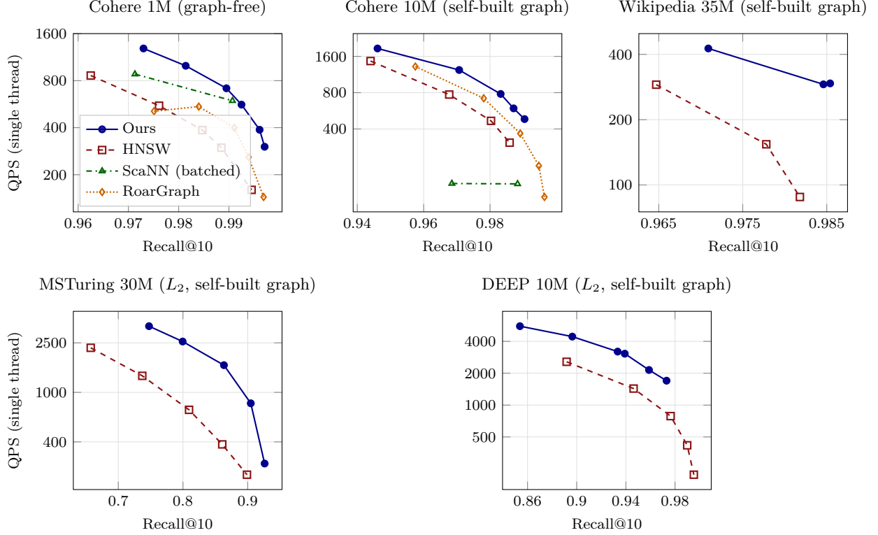
Figure 13: Recall–QPS frontiers (recall@10 versus single-thread queries per second, log scale) on Cohere 1M, Cohere 10M, Wikipedia 35M, MSTuring 30M ( d=100 , L_2 ; ours 2.5\text{--}4\times HNSW, exceeding its 0.899 ceiling), and DEEP 10M ( d=96 , L_2 ; ours \sim 2\times across the measured range, HNSW’s deep tail beyond our sweep’s last point), with both systems measured as same-window sequential pairs; our system runs graph-free at 1M and with self-built graphs at 10M and 35M. At every operating point shown, on all three scales our frontier lies above and to the right of HNSW’s, i.e. higher throughput at equal recall and higher recall at equal throughput; ScaNN (shown batched, favorable to it) and RoarGraph (built in-distribution with 500k base-distributed training queries; 1.6\text{--}2.4\times behind at 1M and 1.2\text{--}1.45\times at 10M — its bipartite projection buys nothing when the query manifold is the base manifold, though it still edges HNSW) trail both. HNSW’s frontier also plateaus at recall 0.9945 (1M), 0.9859 (10M), and 0.9818 (35M), below the recall our system reaches.
