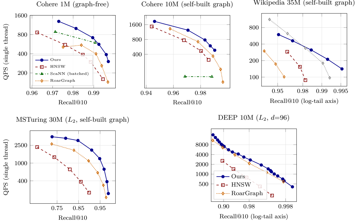
Figure 13: Recall-QPS frontiers (recall@10 versus single-thread queries per second, log scale), showing each method’s warm best-of-repeated frontier. Quoted ratios use same-core sequential pairs; in particular, the DEEP ratios below are strict ABBA/BAAB medians rather than ratios inferred from independently best plotted points. The Wikipedia and DEEP panels use a log-tail recall axis ( \log(1 - \text{recall}) , reversed) so the high-recall contest is resolved rather than compressed into the right edge; on Wikipedia the greyed curve is the build- ineligible 6.5h RoarGraph, the orange curve the gate-eligible budget RoarGraph. Top row (high-dimensional, d \geq 768 ): our regime. On Cohere 1M/10M ( d=768 ) our system leads every baseline — graph-free at 1M, self-built graph at 10M; RoarGraph, though it edges HNSW, is 1.6\text{--}2.4\times (1M) / 1.2\text{--}1.45\times (10M) behind us — its query-aware bipartite projection buys nothing when the query manifold is the base manifold. On Wikipedia 35M ( d=1024 ) we lead every build-eligible baseline across the frontier and reach recall 0.9952 beyond every ceiling; RoarGraph’s shown curve required a 6.5h build ( 3.2\times our 2h gate; our graph self-builds in 10 min) and keeps the 0.93–~0.975 band on that budget — narrowed from above by our 48-edge seeded-NN-descent graph (2.8 h, still under 6.5 h) with the resident stack (0.9778 at 431 QPS under load vs its quiet ~390); a budget-matched RoarGraph ( L=50 , 250k train queries) still takes 3.1h and collapses to a 0.9605 ceiling at ~100 QPS, below our curve everywhere. Bottom row (low-dimensional, d \leq 100 ). On MSTuring 30M ( d=100 ) we beat every baseline at every measured point ( 1.45\text{--}2.8\times RoarGraph, exceeding HNSW’s ceiling); RoarGraph’s curve required padding its input to d=104 — its released code silently corrupts dimensions not divisible by 8. On DEEP 10M ( d=96 ), graph-local physical ordering and corrected-fp16 reranking win the tail, while the portal-SQ4 adaptive walk removes the loose routing+scan toll. Ours beats RoarGraph at every measured point: 1.16\text{--}1.48\times from recall 0.80 to 0.90 against its published curve, and strict same-window medians of 1.156\times at 0.9032, 1.025\times at 0.9265, 1.191\times near 0.943, 1.260\times near 0.960, and 1.303\times at 0.9718, before the corrected-fp16 tail wins 1.379\times at 0.9940 and 1.062\times at 0.9978, then reaches 0.9987 beyond its ceiling.
