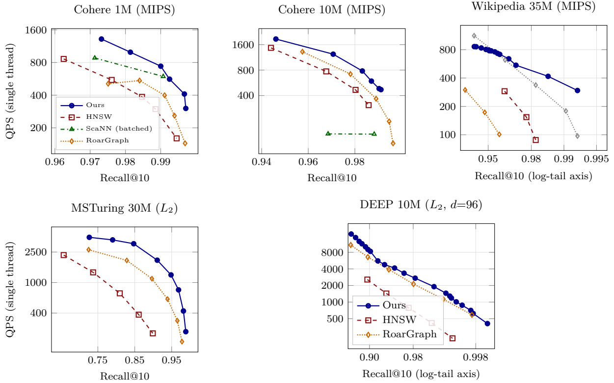
Figure 13: Recall-QPS frontiers (recall@10 versus single-thread queries per second, log scale), showing each method’s warm best-of-repeated frontier. Quoted ratios use same-core sequential pairs; in particular, the DEEP ratios below are strict ABBA/BAAB medians rather than ratios inferred from independently best plotted points. The Wikipedia and DEEP panels use a log-tail recall axis ( \log(1 - \text{recall}) , reversed) so the high-recall contest is resolved rather than compressed into the right edge; on Wikipedia the greyed curve is the build- ineligible 6.5h RoarGraph, the orange curve the gate-eligible budget RoarGraph. Top row (high-dimensional, d \geq 768 ): our regime. On Cohere 1M/10M ( d=768 ) our system leads every baseline using its best eligible configuration; RoarGraph, though it edges HNSW, is 1.6\text{--}2.4\times (1M) / 1.2\text{--}1.45\times (10M) behind us — its query-aware bipartite projection buys nothing when the query manifold is the base manifold. On Wikipedia 35M ( d=1024 ) our plotted curve is a 64-edge graph seeded from the k=16 pass — gate-eligible at 1.46 h total build — with the resident stack: it crosses even the 6.5h build-ineligible RoarGraph near recall 0.953 (0.9531@777 versus \sim 774 ), leads at 0.9566@758 versus \sim 726 , and reaches 0.9677@640 versus \sim 565 , then leads by 1.14\times at 0.972, 1.69\times at 0.986, and 3.0\times at RoarGraph’s 0.9925 ceiling. It concedes only 0.93\text{--}0.953 (up to \sim 1.3\times at 0.933, narrowing to parity by 0.953) — an eligible-vs-ineligible comparison; a budget-matched RoarGraph ( L=50 , 250k train queries) still takes 3.1h and collapses to a 0.9605 ceiling at \sim 100 QPS, below our curve everywhere. Bottom row (low-dimensional, d \leq 100 ). On MSTuring 30M ( d=100 ) we beat every baseline at every measured point ( 1.45\text{--}2.8\times RoarGraph, exceeding HNSW’s ceiling); RoarGraph’s curve required padding its input to d=104 — its released code silently corrupts dimensions not divisible by 8. On DEEP 10M ( d=96 ), graph-local physical ordering and corrected-fp16 reranking win the tail, while portal-SQ4 entry plus budgeted local refinement removes the loose routing+scan toll. Fixed rounds replace best-first above recall 0.80 and add 6.1\text{--}17.4\% strict median QPS at matched recall; a direct pair at 0.9032 is 1.265\times RoarGraph ( 1.204\times best-to-best). Ours beats RoarGraph across the loose curve and by strict same-window medians of 1.19\text{--}1.38\times from 0.943 through 0.994, reaching 0.9987 beyond its ceiling; the 0.9265 join shoulder and the 0.9978 point remain inside RoarGraph’s demonstrated \sim 1.2\times window-phase swing and are marked parity pending multi-window confirmation; the 0.9032 join point itself is confirmed across three window-separated quiet ABBA rounds (medians 1.09\times , never behind under any symmetric convention).
