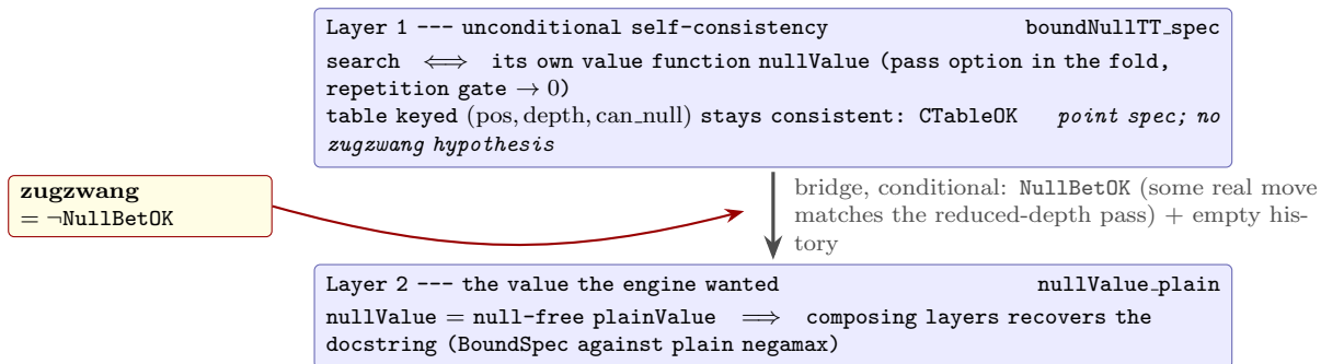
Figure 7: The layered null-move argument (Section 15.1). The unconditional layer proves the search and its keyed table can never disagree with each other ; the named hypothesis NullBetOK is confined to the bridge that identifies the computed value with the null-free one. Zugzwang attacks only the bridge — it can make the value wrong, never the table inconsistent.
