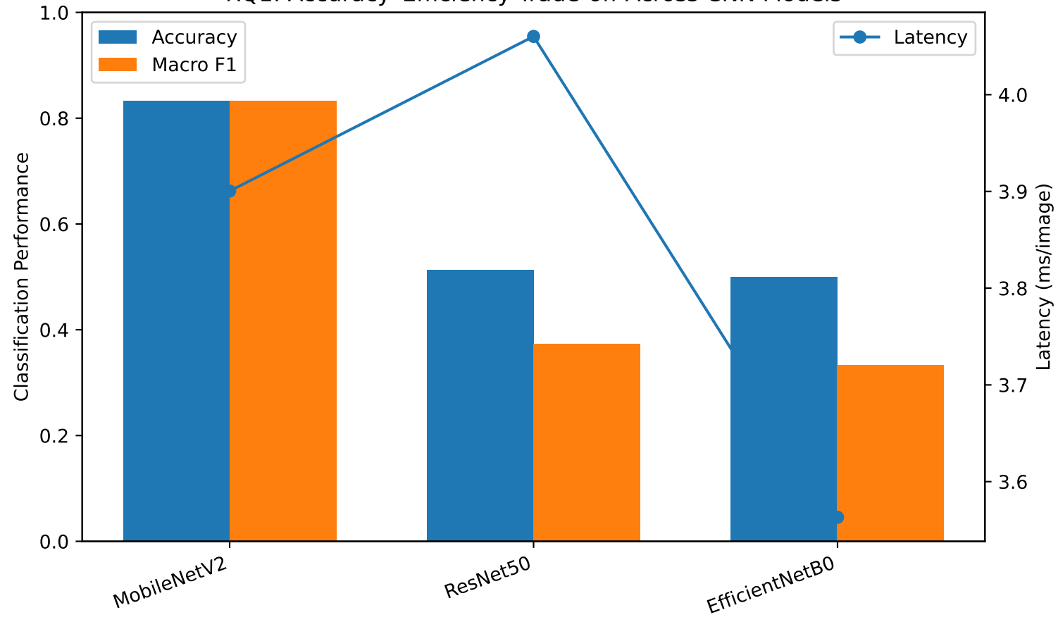
RQ1: Accuracy-Efficiency Trade-off Across CNN Models
