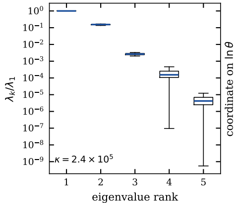
(a) normalized FIM spectrum
