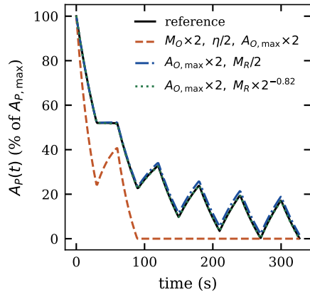
(c) forward simulation, protocol B
