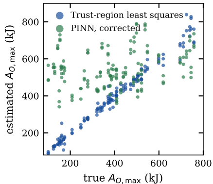
(a) shrinkage of A_{O,\max}
