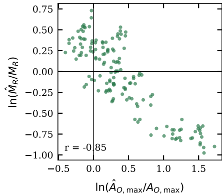
(b) error along the flat direction
