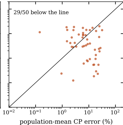
Differential Evolution
