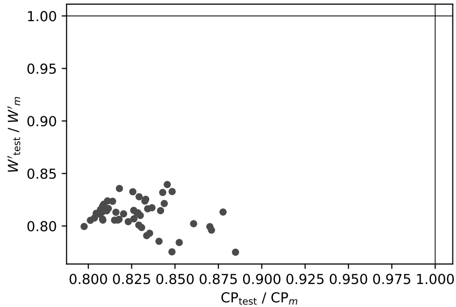
(b) two-parameter fit on model trials, 50 athletes
