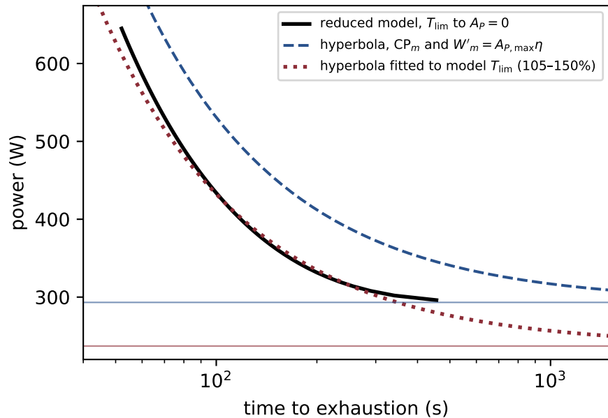
(a) power-duration relation, median athlete
