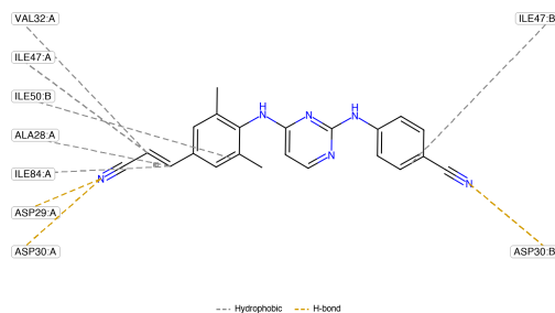
Figure 14. SDF-aware PLIP interaction diagram for Rilpivirine, energy rank 3, cluster 1 (Vina score -8.282 kcal/mol). Ligand bond orders, aromaticity, formal charges, and stereochemistry come from the retained pose SDF; interaction calls come from the retained PLIP report.xml. The PLIP XML/text files remain the authoritative interaction records.
